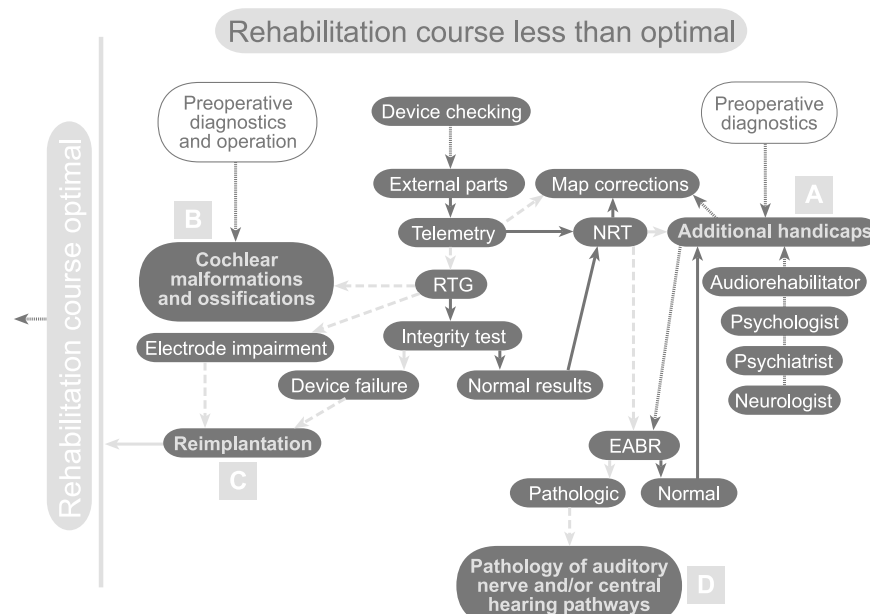
Fig. 1 Diagnostic algorithm.
